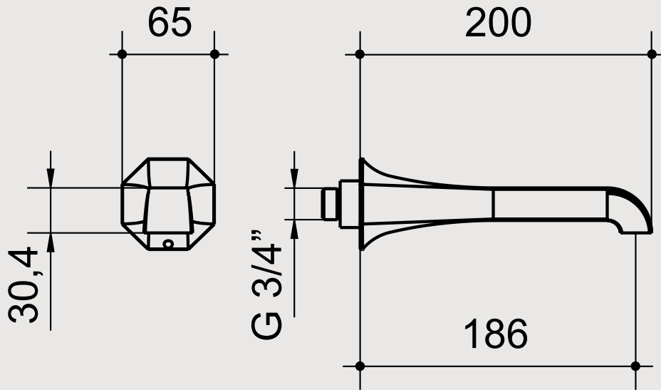
BL320 - Spout
